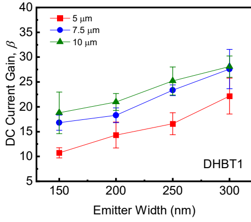
(a) \beta scaling behavior in DHBT1.
