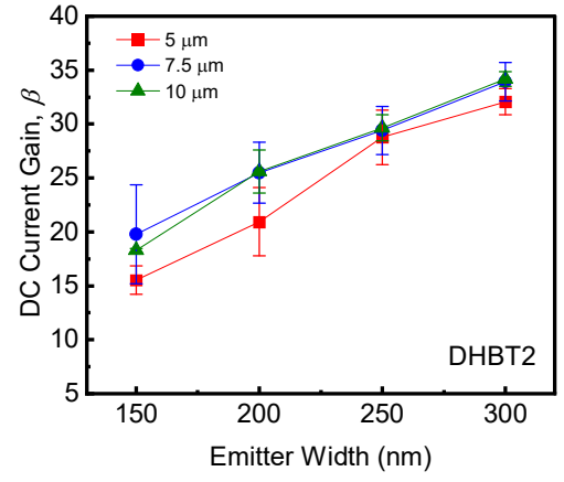
(b) \beta scaling behavior in DHBT2.
