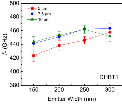
(c) f_T scaling behavior in DHBT1.
