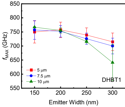
(e) f_{MAX} scaling behavior in DHBT1.
