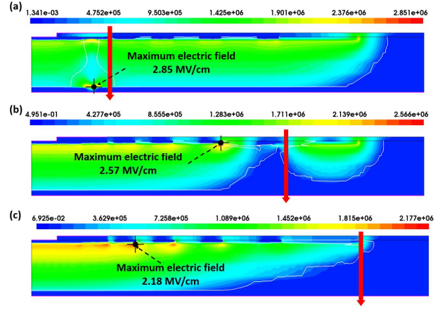
Fig. 8. Electric field distributions in the RA-JTE structure for various lateral strike locations of (a) main junction, (b) last P + ring, and (c) end of the JTE region under a drain bias of 1200 V.
